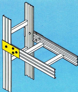
VERTICAL BRANCH PLATE
