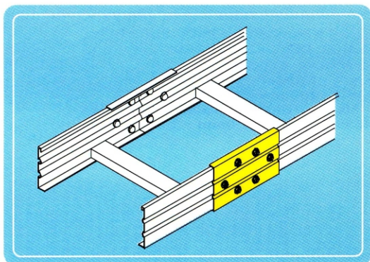
STRAIGHT CONNECTOR
