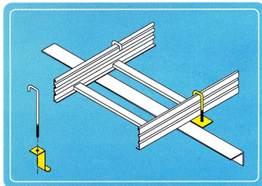
OUTSIDE HOOK BOLT
