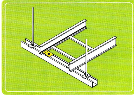
INSIDE HOLD DOWN CLAMP
