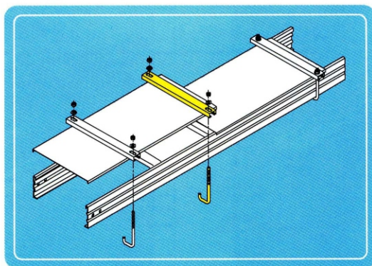
U-COVER CLAMP
