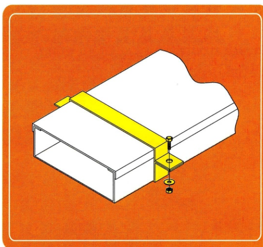
ㄇ型蓋板夾 ㄇ-COVER CLAMP
