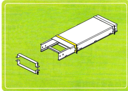
ㄇ-COVER CLAMP
