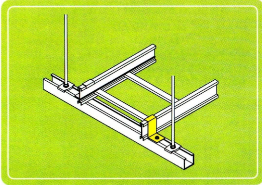
OUTSIDE HOLD DOWN CLAMP
