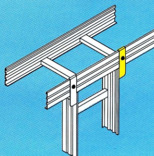
SIDE PATH BRANCH PLATE
