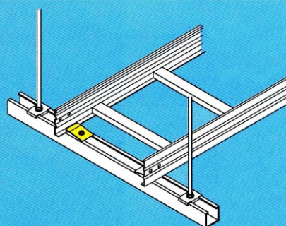
INSIDE HOLD DOWN CLIP
