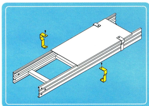
SIDE COVER CLAMP
