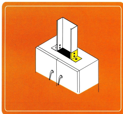
配電盤連接片 PANNEL SPLICE PLATE
